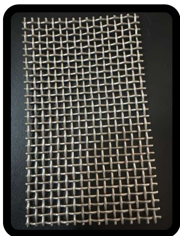
MESH 10 X 10 R CAL 21 ABERT 1.727 MM
