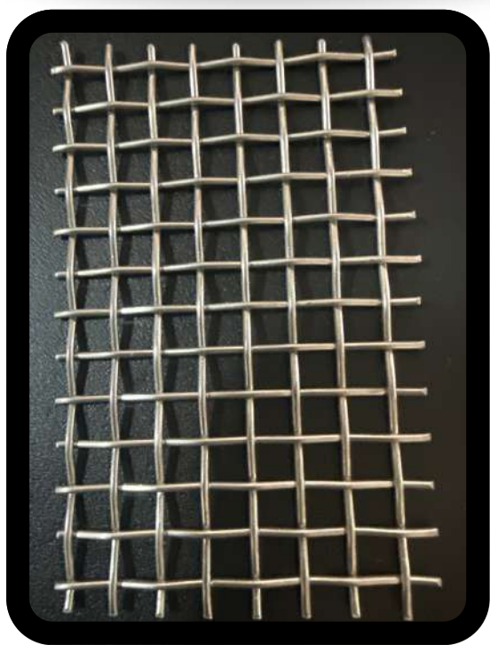
MESH 5X5 CAL 20 ABERT 4.191 MM
