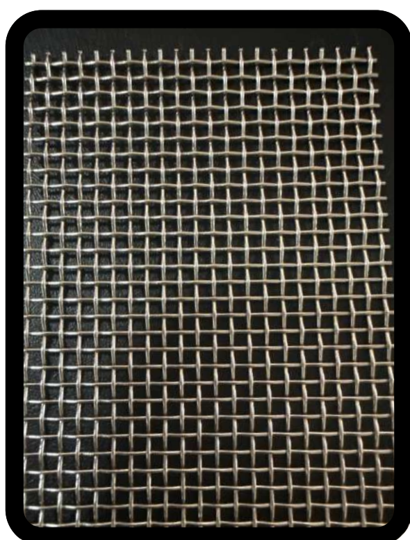
MESH 12X12 CAL 24 ABERT 1.549 MM
