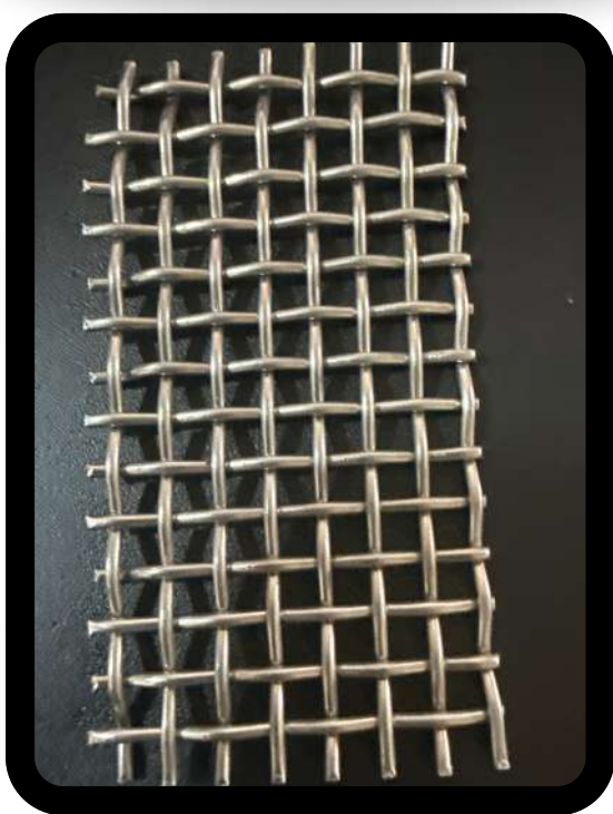
MESH 6X6 R CAL 18 ABERT 3.048 MM
