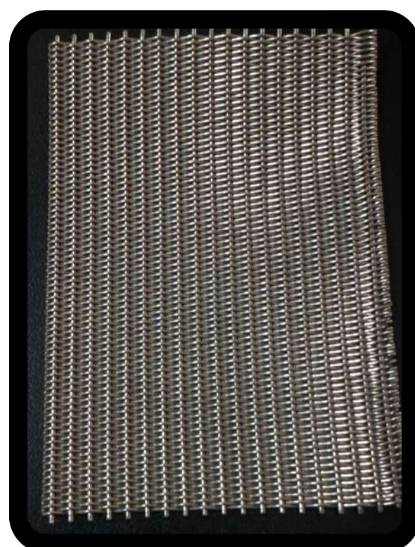
MESH 12 X 64 CAL 23/27 ABERT 0.27 MM
