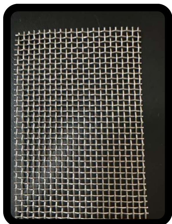
MESH 14X14 CAL 25 ABERT 1.295 MM
